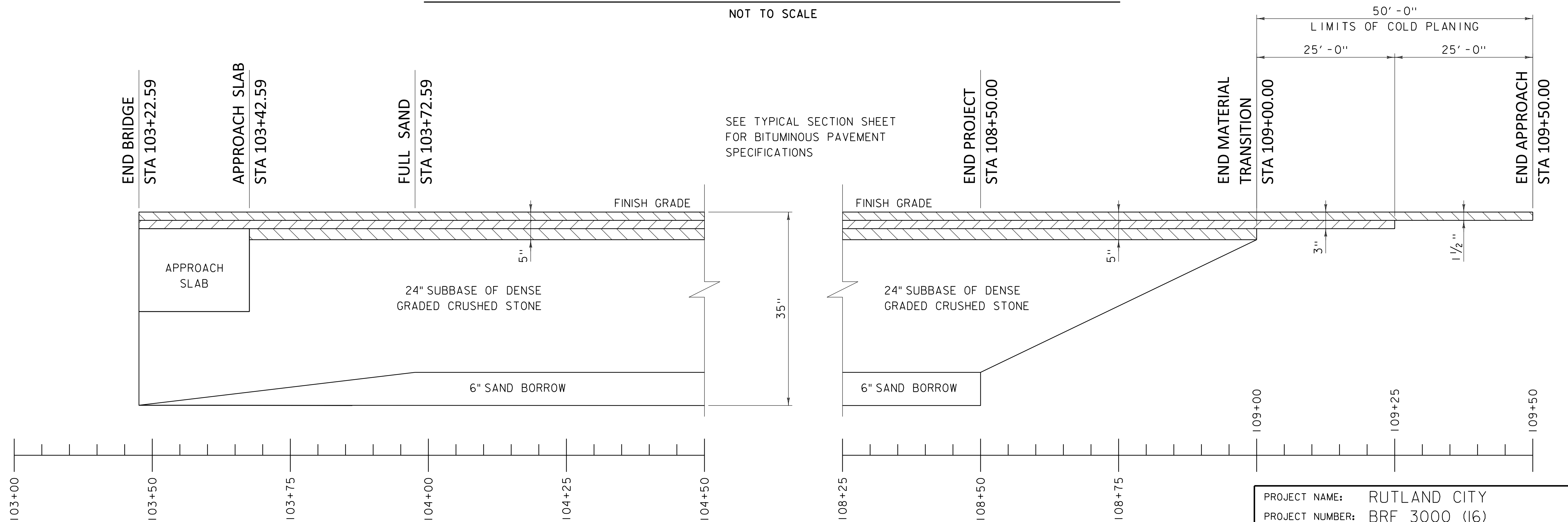
TH-8 (RIVER STREET) MATERIAL TRANSITION DETAIL
