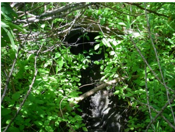
Outfall 74: 12" CMP
