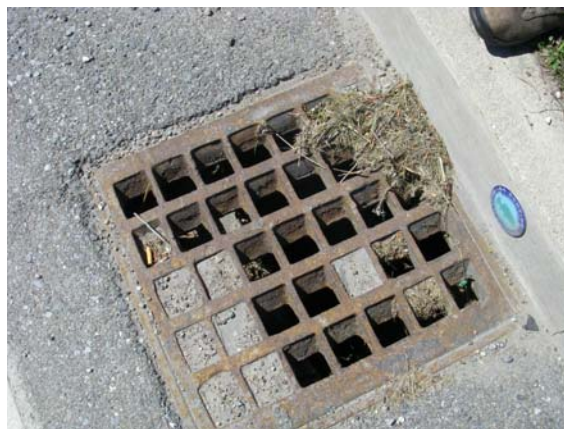
Outfall 315: 15" PVC
