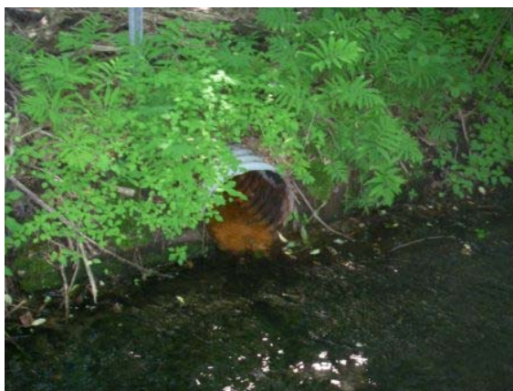
Outfall 5: 18" CMP
