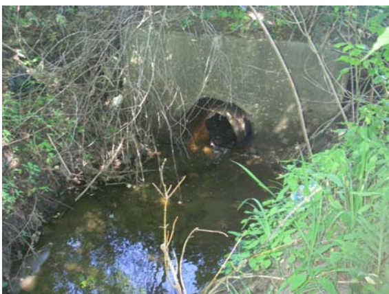
Outfall 258: 18" CMP
