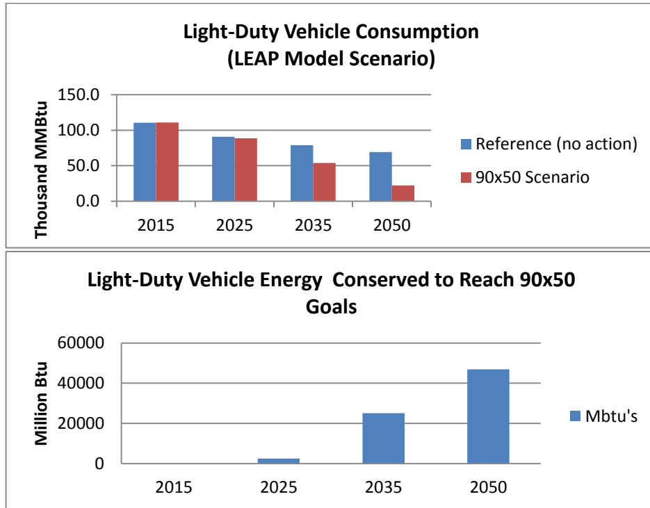
Figure 6: Reference vs 90x50 scenario; the amount of energy to be conserved over the benchmark years.
