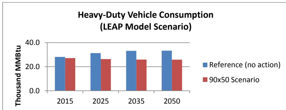
Figure 7: LEAP model scenario for Heavy-duty vehicle energy consumption over the benchmark years.
