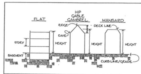
Figure 1 BUILDING HEIGHT
