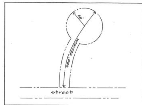
Figure 2 CUL-DE-SAC STREET
