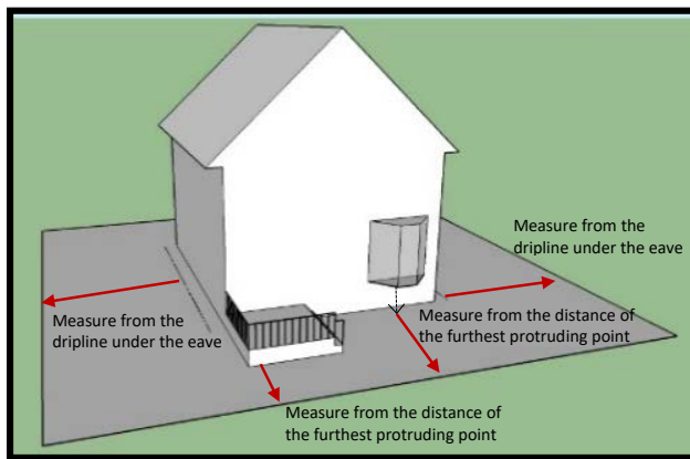
Figure 2.2. Measuring Setbacks
