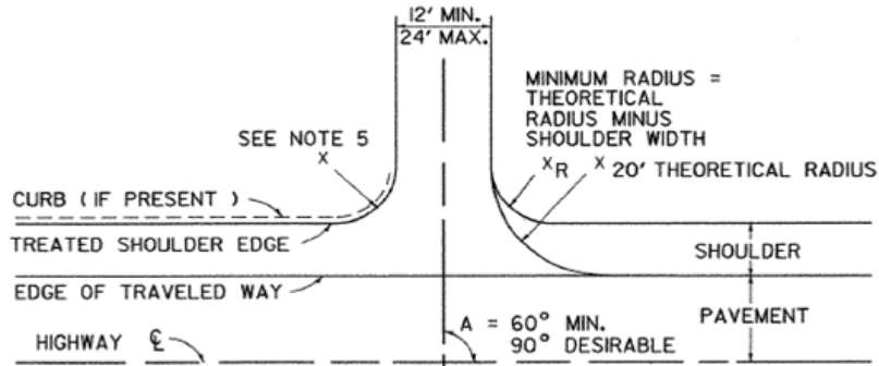
Figure 5.1 – B-71 Standards for Residential Drives (VTrans)
