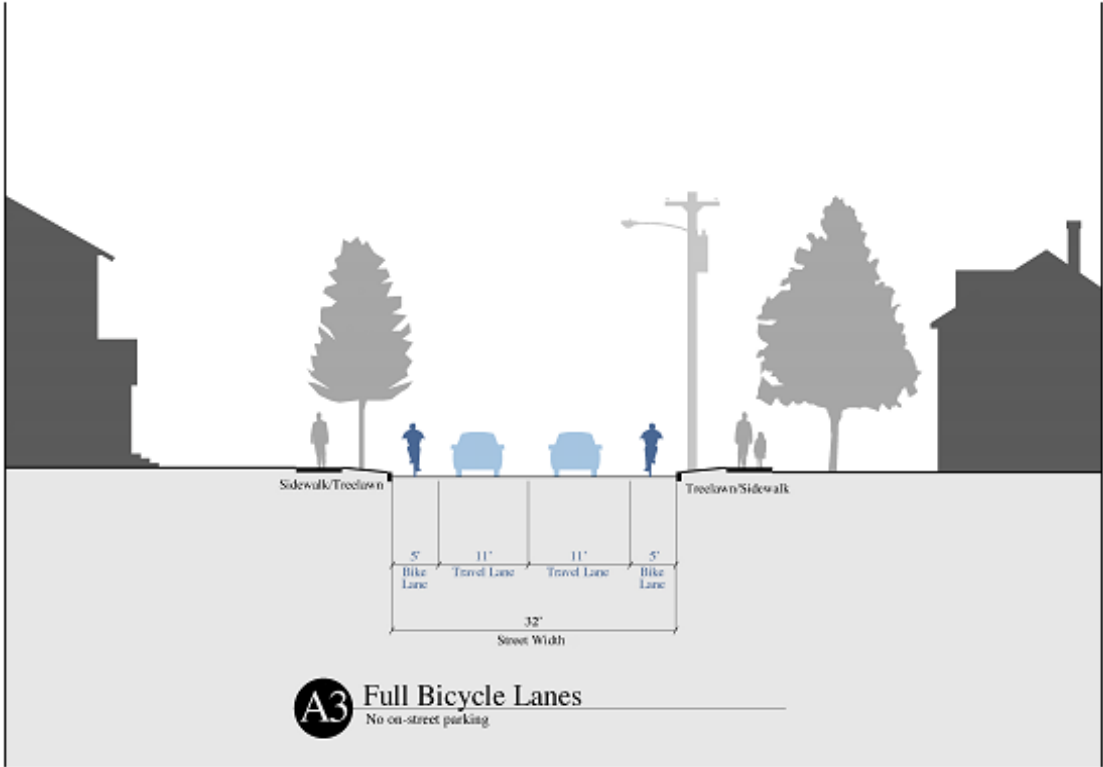
Figure 20 A3 – Typical Section through a Montpelier Street
